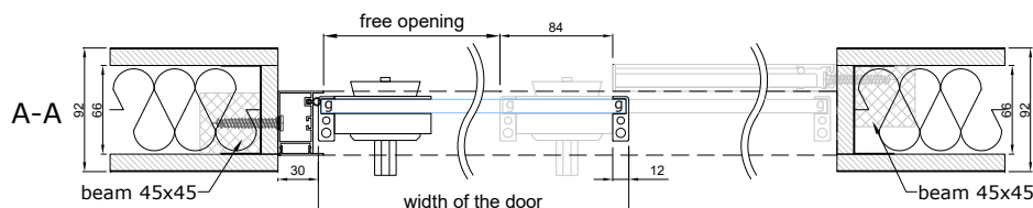
CONNECTION WITH WALL (WITH LOCKING AND/OR PULL HANDLES)
