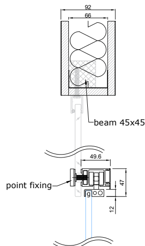
DECOR PROFILES ARE GLUED ON BOTH SIDES OF THE GLASS
