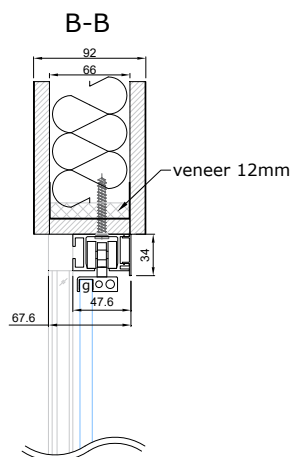
CONNECTION WITH CEILING
