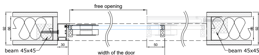
CONNECTION WITH WALL (BUILT-IN HANDLES AND WITHOUT LOCKING)
